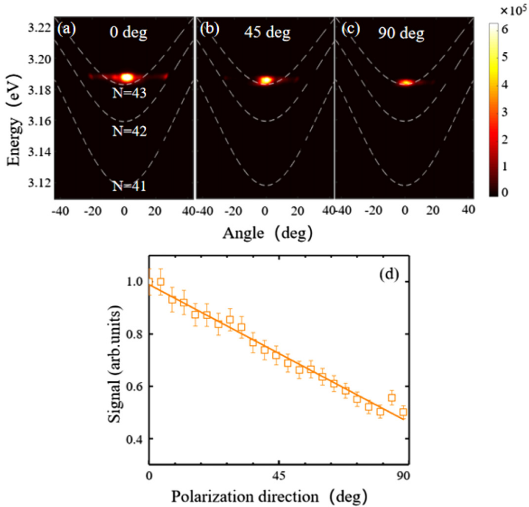
Figure 2. (a)–(c) Static-state k -space angle-resolved PL mappings for polariton condensates under excitation pulses along three different polarization directions. The dispersion curves (indicated by the white dashed curves) are obtained from fitting with the classical plane waves model. (d) The excitation polarization dependence of the condensation signal at a fixed pump power of 0.8 \mu\text{W} . The solid line is from a linear fitting.
