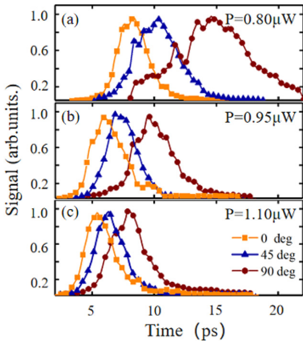
Figure 4. The polarization dependence of polariton condensate dynamics at pump powers of (a) P = 0.80 \mu\text{W} (b) P = 0.95 \mu\text{W} (c) P = 1.10 \mu\text{W} . As P increasing, the time interval shrinks. For a better quality of the figure, only 10% of the measured data points are shown here.
